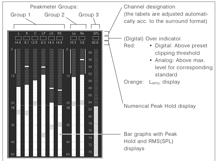
Fig. 1-5: Display elements of the Peak Program Meter instrument (PPM) in Surround mode
