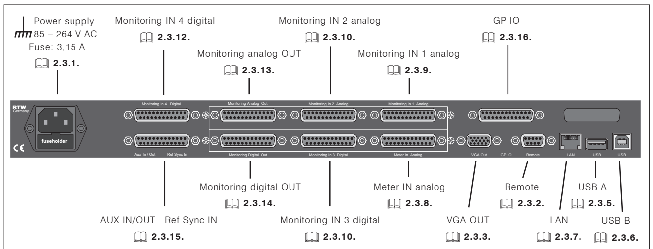
Fig. 2-2: Connectors on the rear panel of the SurroundControl 30900(-24)
