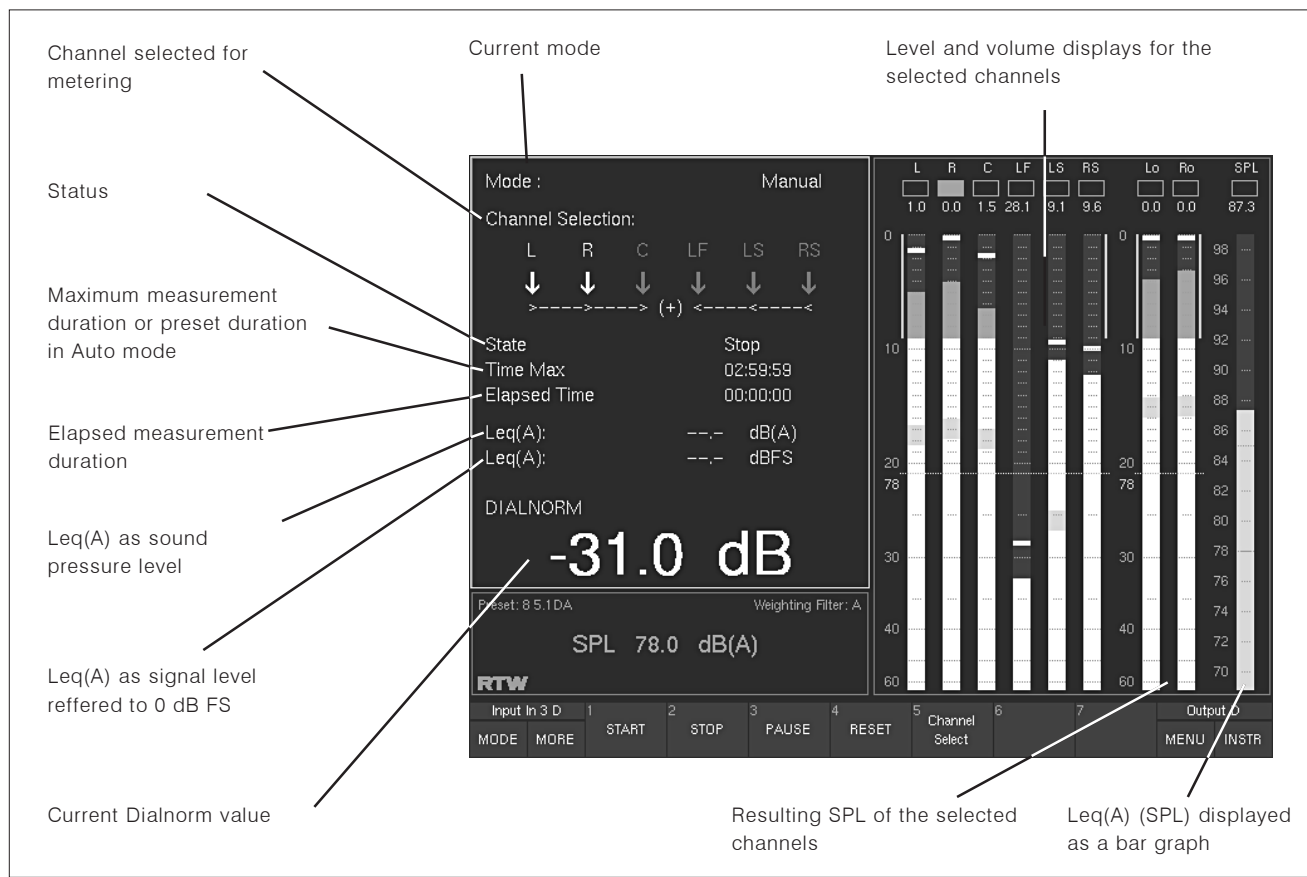
Fig. 1-17: The Dialnorm instrument (DIALNORM)
