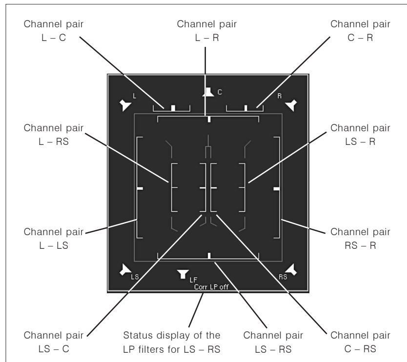
Fig. 1-11: The Correlator instrument (COR) as multi correlator in Surround mode
