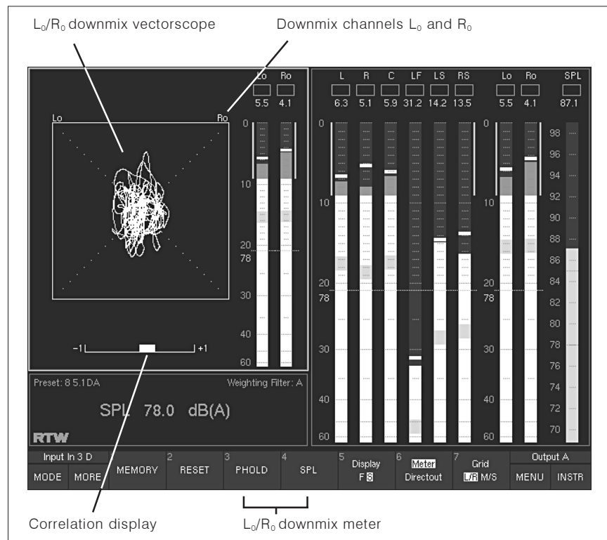
Fig. 1-15: The (Two-Channel) Downmix Meter instrument (DOWNMIX)
