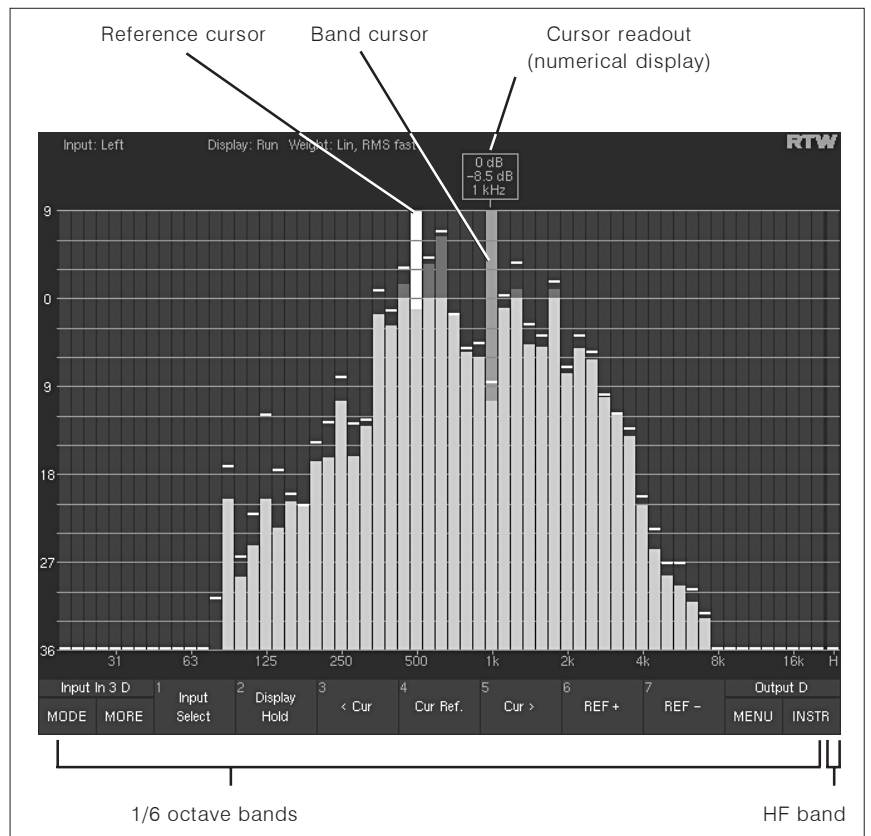
Fig. 1-14: The 1/6 octave RTA instrument (RTA 1/6)
