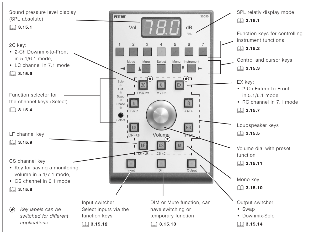
Fig. 3-29: The controls of the Remote Control 30050
