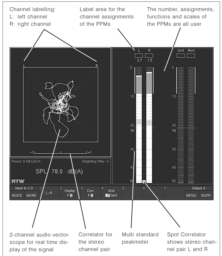
Fig. 1-10: The Audio Vectorscope instrument (VSC) in 2 Channel Stereo mode (L and R channel mode)
