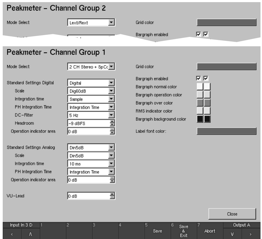
Fig. 4-37: The menu pages of the channel groups available in 2 Channel Stereo mode
