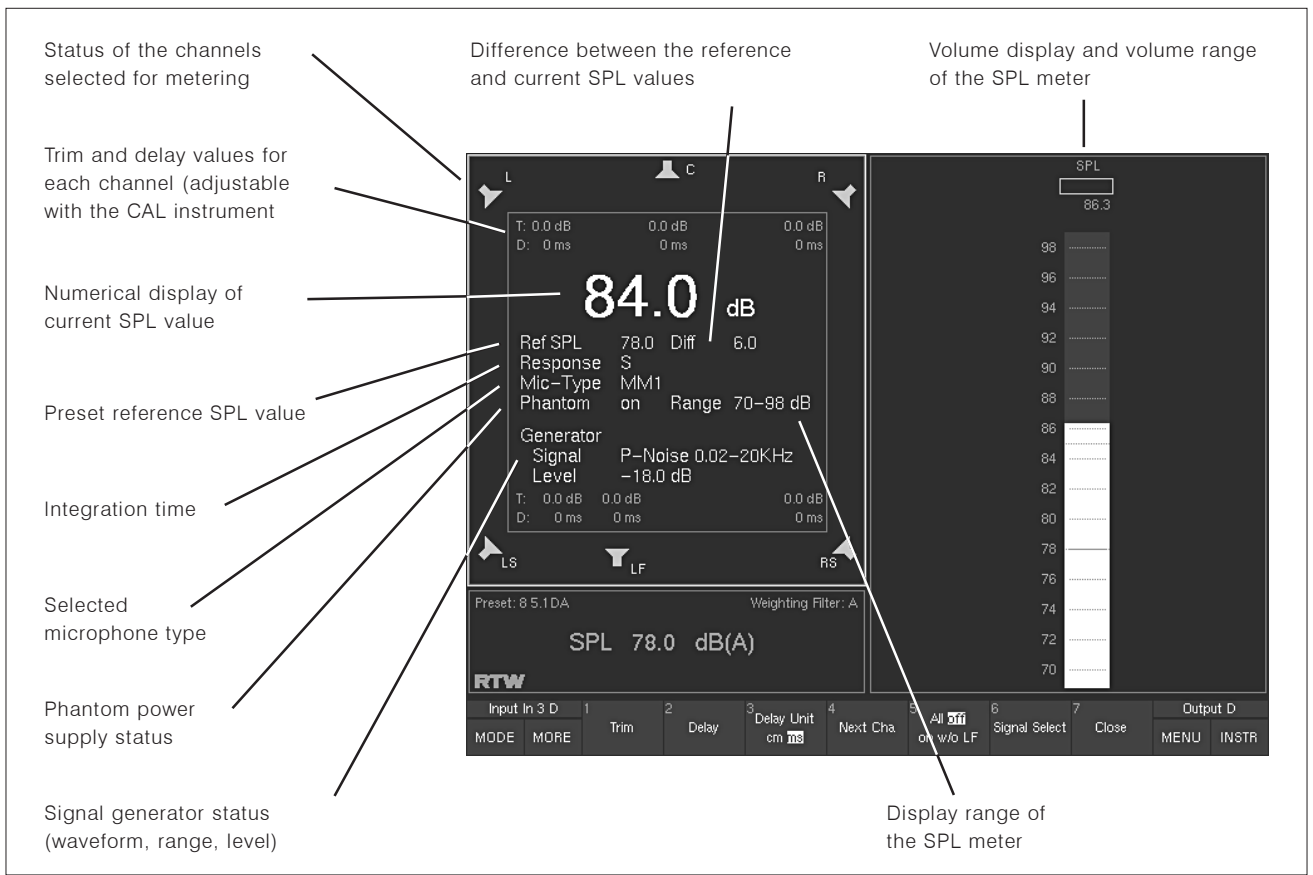
Fig. 1-19: The CAL (Calibration) instrument
