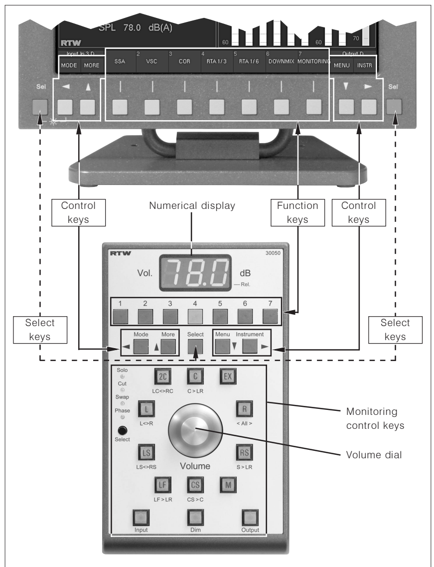
Fig. 3-1: The SurroundControl 30900(-24) controls
