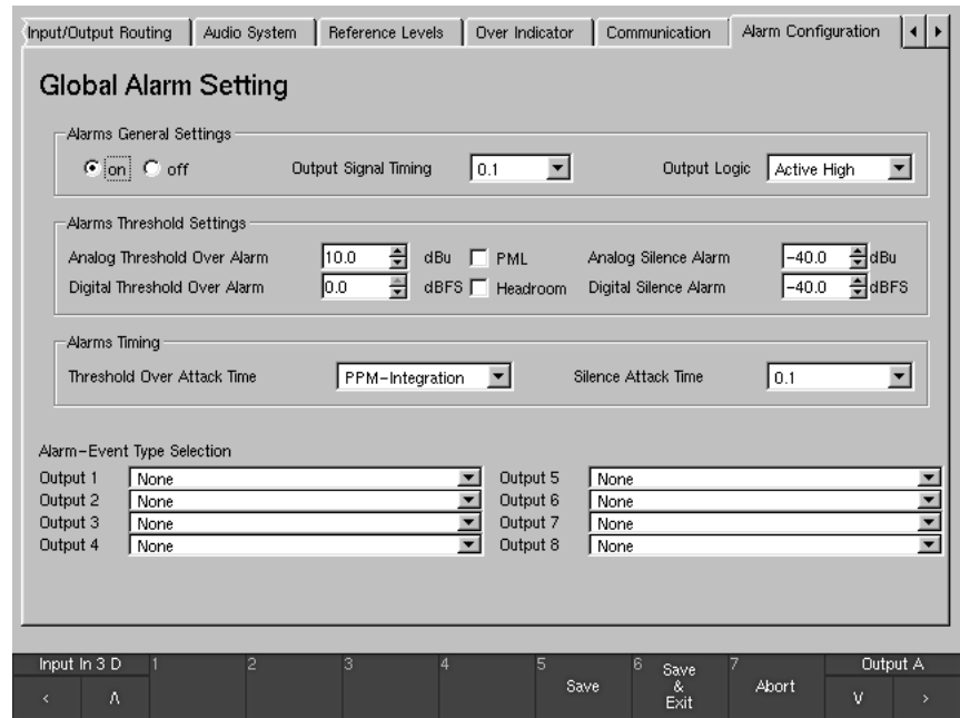
Fig. 4-26: The Alarm Configuration menu tab in Surround mode
