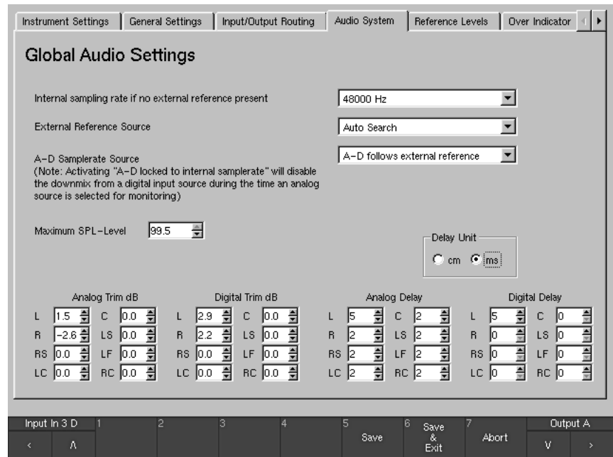
Fig. 4-20: The Audio System menu tab
