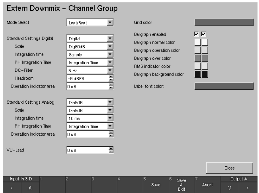
Fig. 4-36: The Extern Downmix - Channel Group menu page
