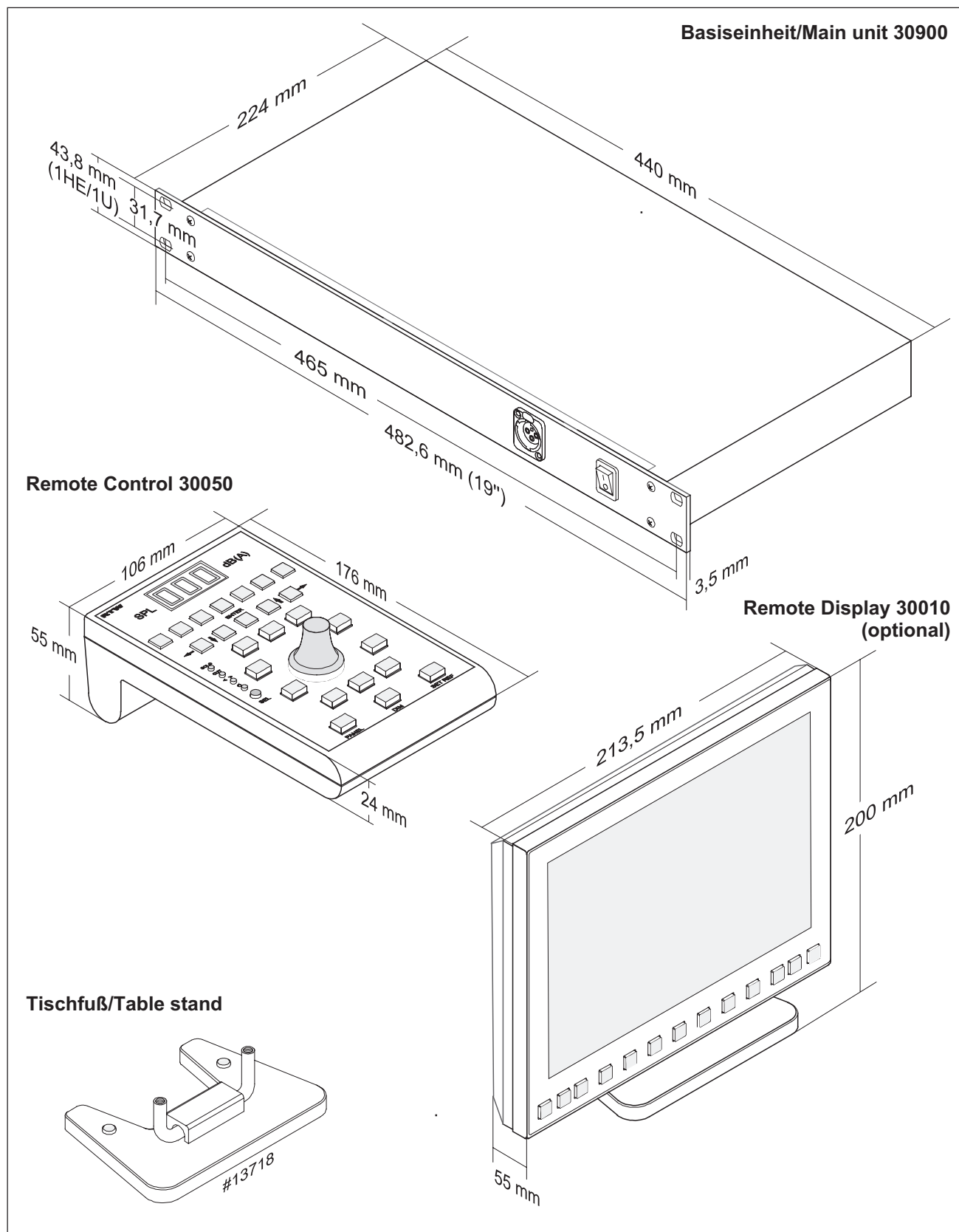
Fig. 6-1: Dimensions of the SurroundControl 30900(-24) system
