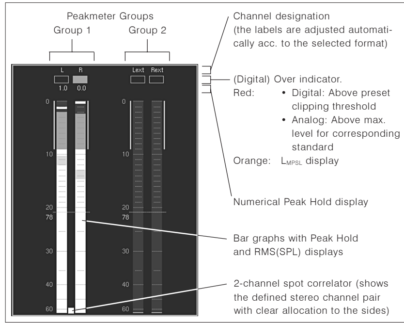
Fig. 1-6: Display elements of the Peak Program Meter instrument (PPM) in 2 Channel Stereo mode
