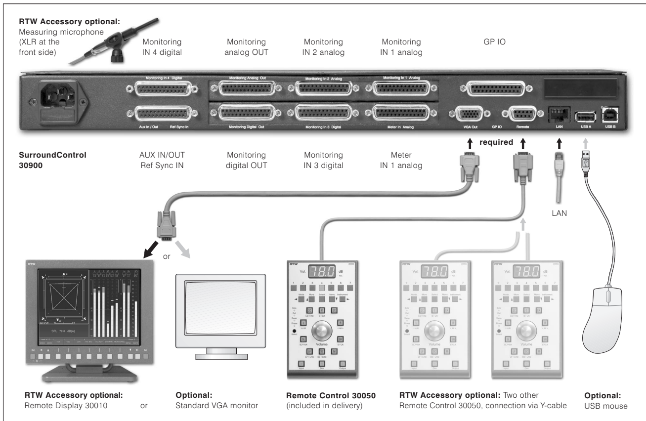
Fig. 6-2: Overview of the configuration of the SurroundControl 30900(-24) system
