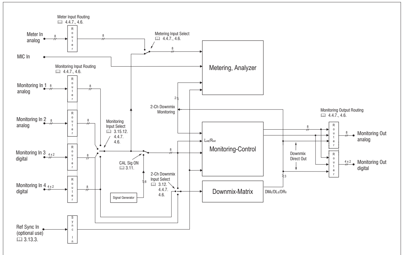
Fig. 4-2: Signal routing in the SurroundControl 30900(-24)
