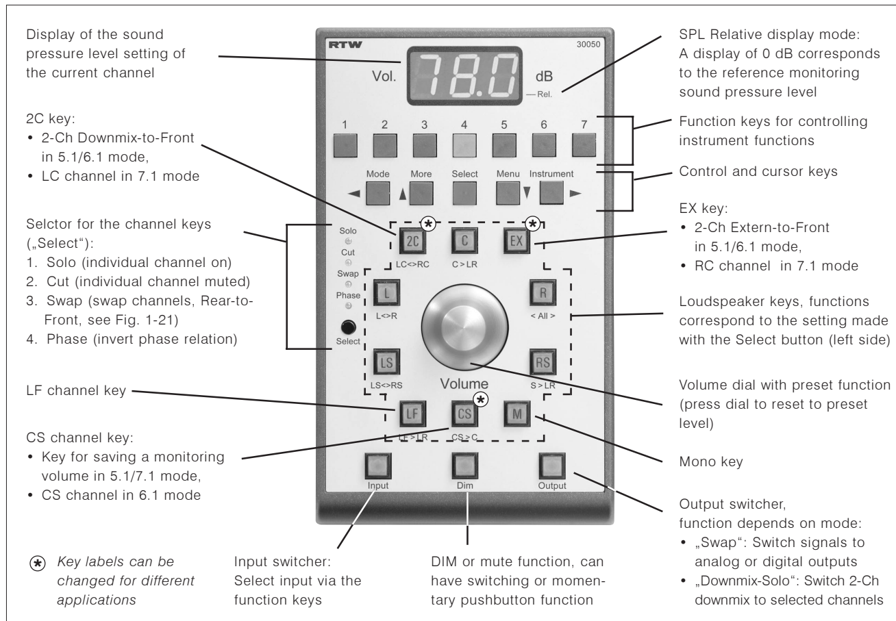
Fig. 1-20: Function keys of the Remote Control 30050
