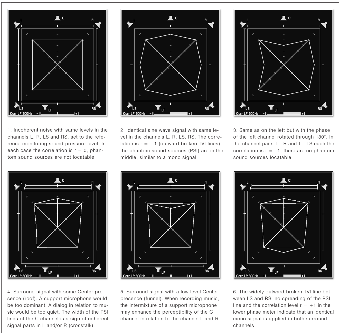
Fig. 1-8: Examples of displays in the Surround Sound Analyzer instrument (SSA), also see: www.rtw.de/english/special/index.html
