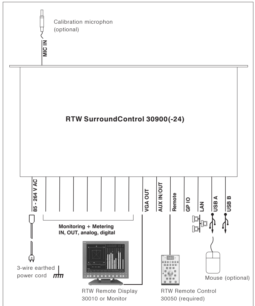
Fig. 2-1: Schematic representation of the unit's connections
