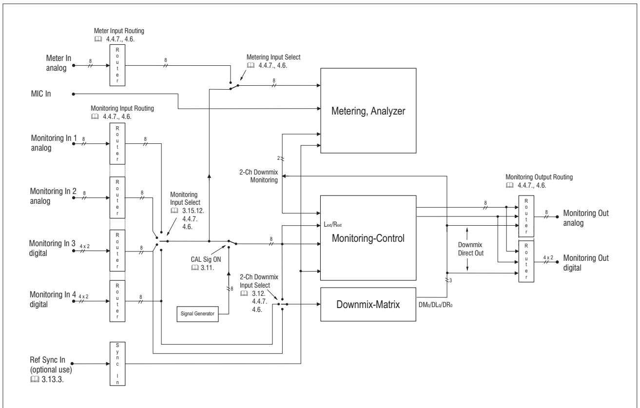
Fig. 2-3: Information flowchart SurroundControl 30900(-24)
