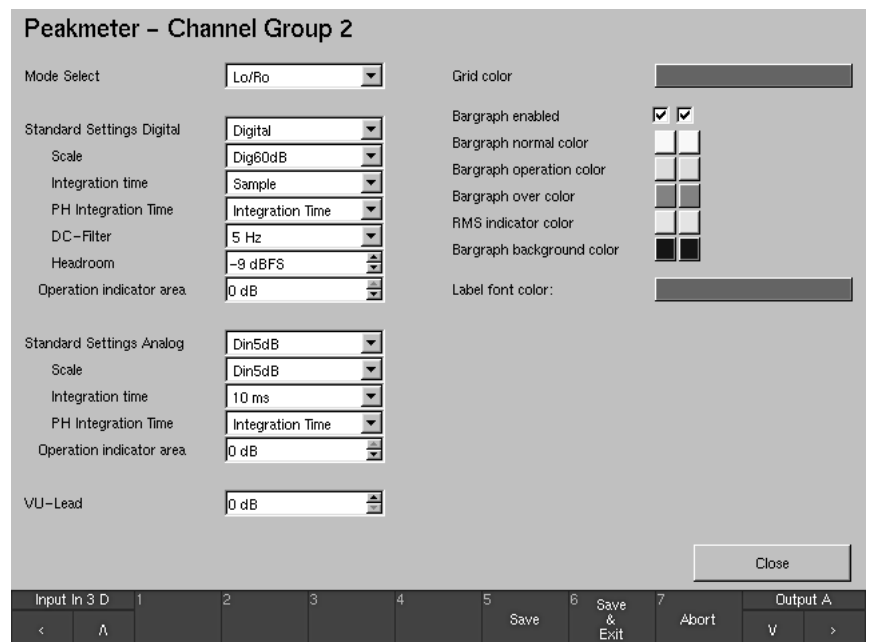
Fig. 4-33: The Peakmeter - Channel Group 2 menu page
