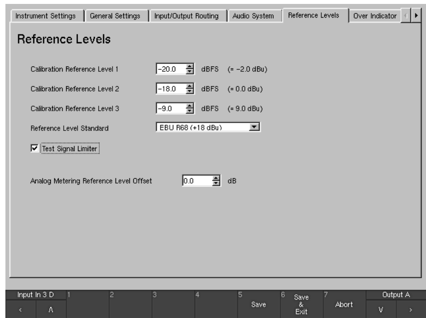
Fig. 4-23: The Reference Levels menu tab
