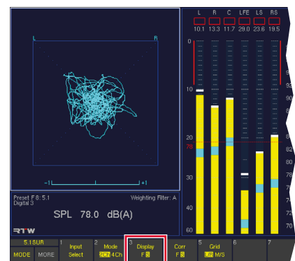
5 Vectorscope in Function Select mode
