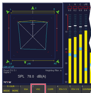
3 Instrument Select mode
